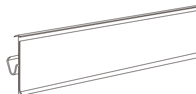
31206 Data strip Material: PVC Label height: 40mm Different length and color available
