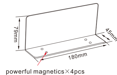
20038 Acrylic sign holder powerful magnetics Material: Acrylic
