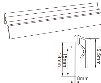
31223 Data strip Material: PVC Different length and color available
