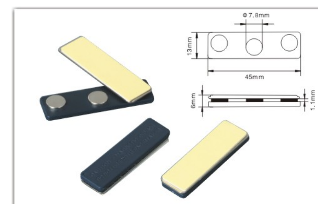
30323-A 证件袋磁铁贴 Rectangular shape adhesive magnet set, use for badge holder, with three pieces strong magnet attached
